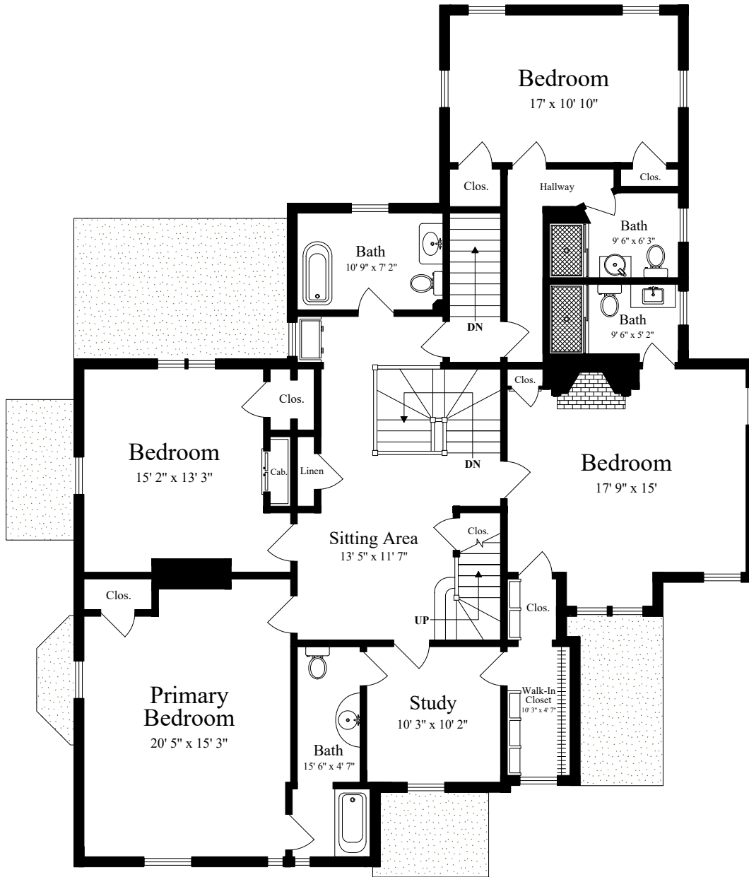
SECOND FLOOR (ceiling = 9')
