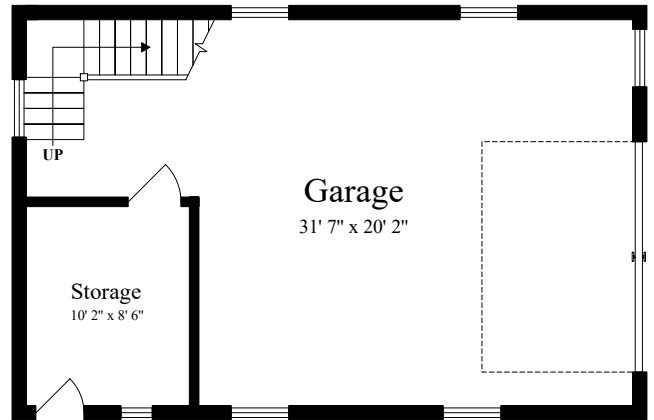
FIRST FLOOR/Carriage House (ceiling = 9' 10")
